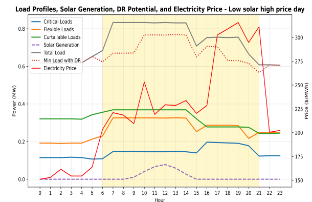
Fig. 10. Data analysis of February 6, 2015 (low solar high price)
