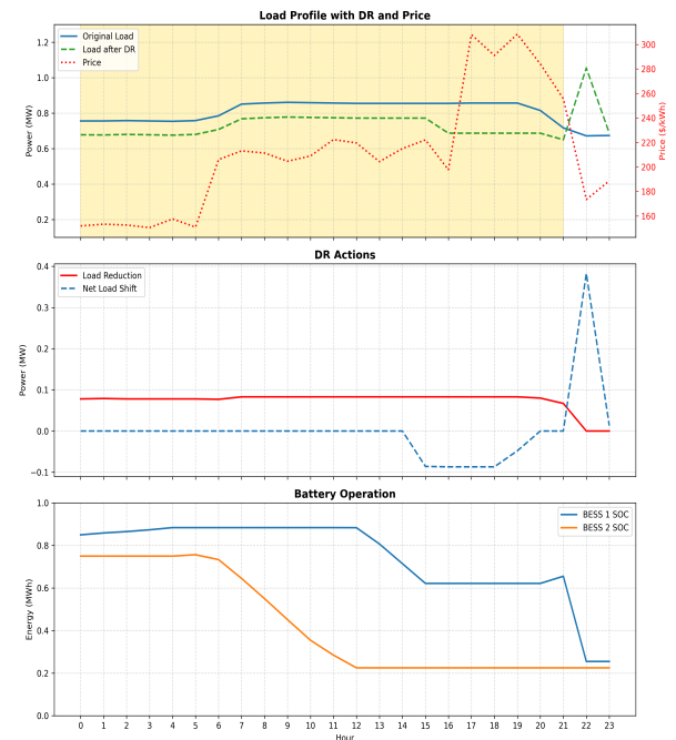
Fig. 7. Optimization results of December 30, 2014 (high demand day)
