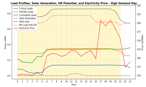
Fig. 6. Data analysis of December 30, 2014 (high demand day)
