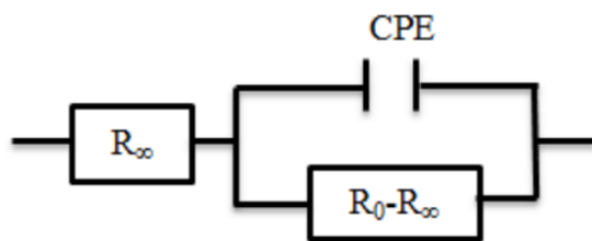
Fig. 5. Cole-Cole impedance model
