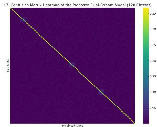
Fig. 7. Confusion matrix (heatmap) of the proposed dual-stream model on the test set
