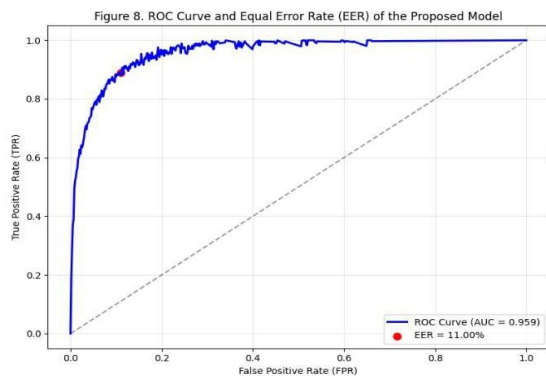
Fig. 8. Receiver Operating Characteristic (ROC) curve and EER of the proposed dual-stream model on the test set
