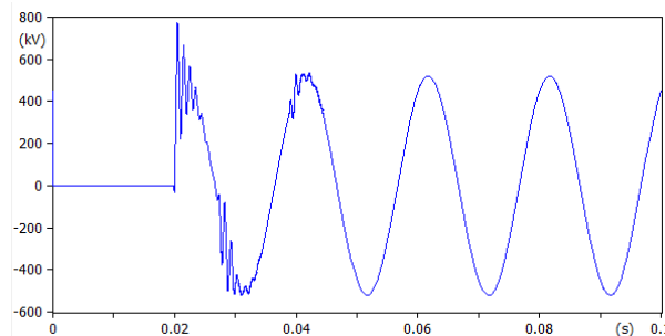
Fig. 15. Phase-A TRV after applying both the surge arrester and neutral-grounding disconnecter
