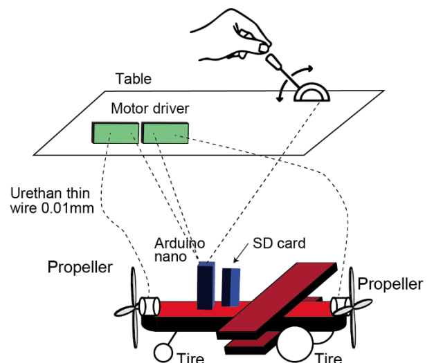
Fig. 4. Manual control (thrust command from the potentiometer)
