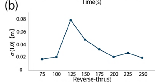
Fig. 8. (a) Summary of Experiment 1(b). (b) Follow-up experiment varying the fixed reverse-thrust level to reassess dispersion in the final position
